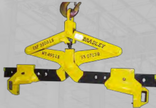
ADJUSTABLE END GRIP BILLET TONG
