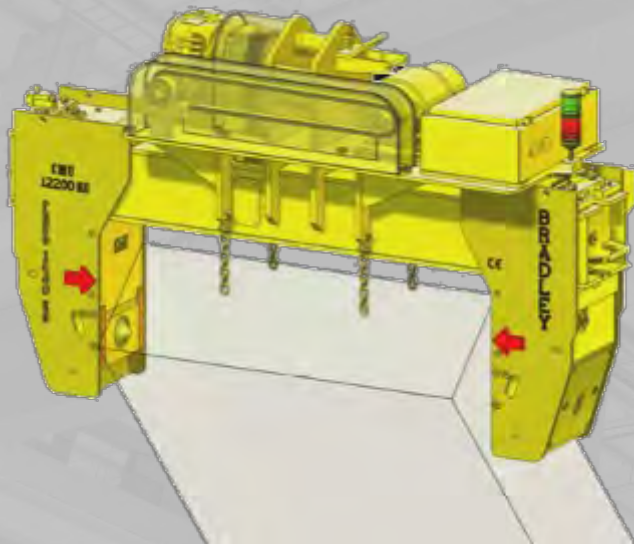
MOTORIZED INGOT SWIVEL GRAB
